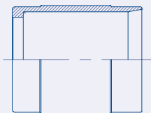
NON SKIVE Balfit® PTFE Convuluted Ferrule 20.TFC
