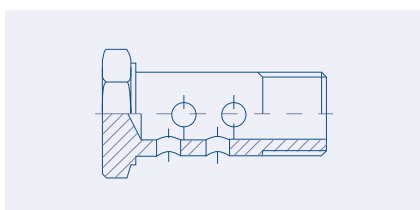
BSP Banjo Double Bolt
