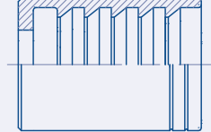
NON SKIVE Balfit® 2 Wire Braid Ferrule 20.201 / 20.302
