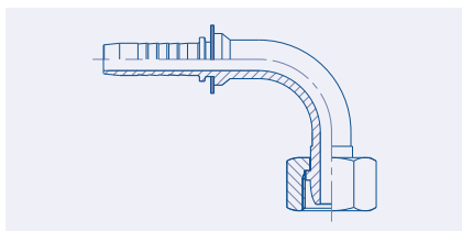
90° Swept Female Metric 24°/60° Cone Seat Swivel (DKL)
