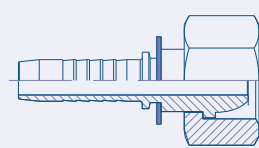
Female Metric 24°/60°C one Seat Swivel (DKL) 23.5213
