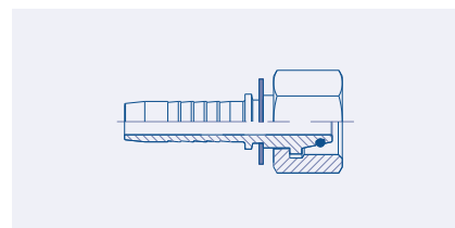
Female Metric French Serie 24° Cone Seat Swivel (DKF)
