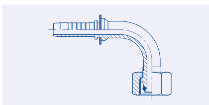
90° Swept Female Metric French Serie 24° Cone Seat Swivel (DKF)
