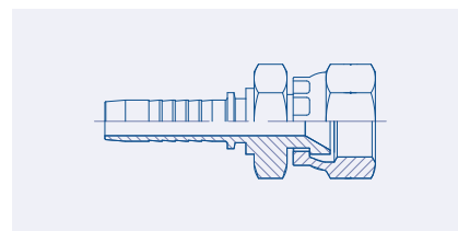
Female JIS 60° Cone Seat Swivel (KOMATSU)
