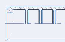
NON SKIVE Balfit® Textile Braid, Thermoplastic & PTFE Ferrule 20.107
