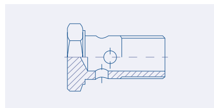
BSP Banjo Bolt
