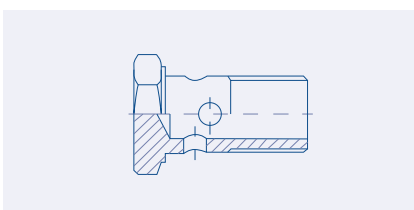
Metric Banjo Bolt
