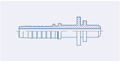
Balwash Standpipe wit O-ring (Karcher) 23.6214
