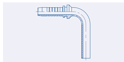
90° Swept Metric Standpipe (BEL 90)
