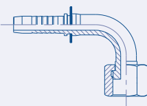
90° Swept Female ORFS Swivel 23.4494
