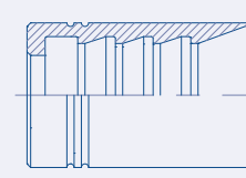
EXTERNAL SKIVE Balfit® 2 Wire Braid & 4 Spiral Ferrule 20.200
