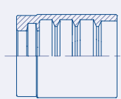
NON SKIVE Balfit® 1 Wire Braid Ferrule 20.305
