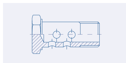
Metric Banjo Double Bolt
