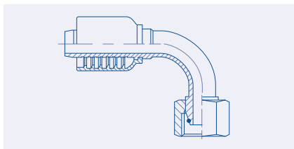
Light 24° Metric 90° Elbow Female - DLF90
