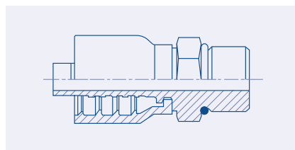
SAE Straight O-ring Boss Male - RA
