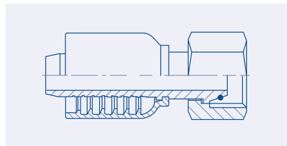
Heavy 24° Metric Female - DHF
