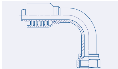
Female JIC 37° Swivel 90° Long Elbow - FJ90L
