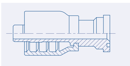
Straight SAE 3000 PSI Code 61 Flange - PA
