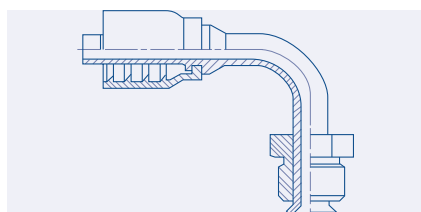
SAE Inverted 45° Flare 90° Elbow Male - MSAE 90
