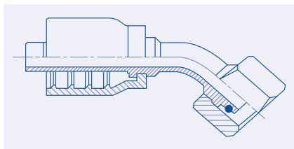
Heavy 24° Metric 45° Elbow Female - DHF45
