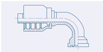
90° Elbow SAE 6000 PSI Code 62 Flange - PH90
