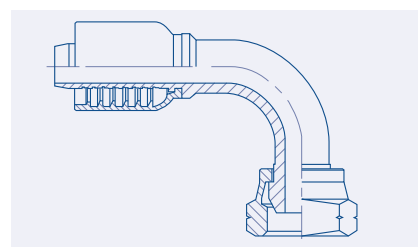
BSP 60° Swivel 90° Elbow Female - BSPXF90
