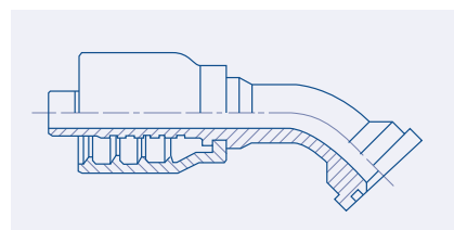
45° Elbow SAE 3000 PSI Code 61 Flange - PA45
