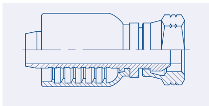
Female NPSM Pipe Swivel - FPX
