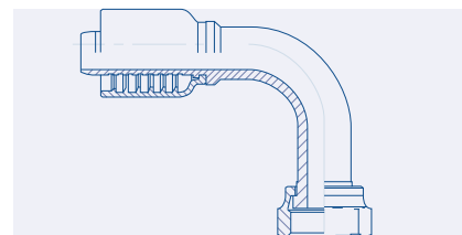
Female ORFS Swivel 90° Long Elbow - OFT90
