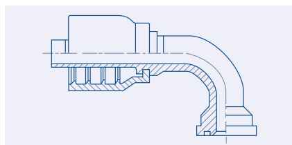
90° Elbow SAE 3000 PSI Code 61 Flange - PA90
