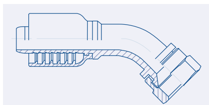
Female SAE 45° Swivel 45° Elbow - FX45
