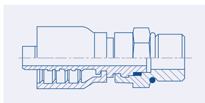
SAE Straight Swivel O-ring Boss Male - RAX
