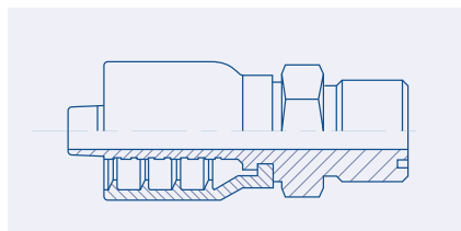
Male ORFS - OFTM
