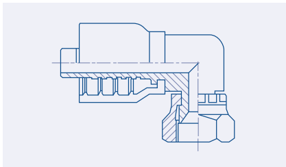
Female JIC 37° Swivel 90° Short Elbow - FJ90S
