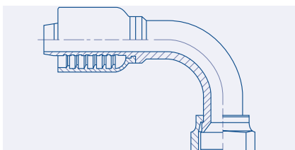
Female SAE 45° Swivel 90° Elbow - FX90
