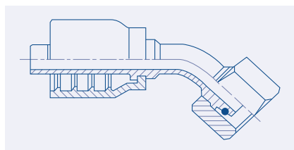
Light 24° Metric 45° Elbow Female - DLF45
