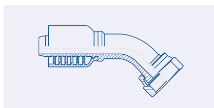
Female ORFS Swivel 45° Elbow- OFT45
