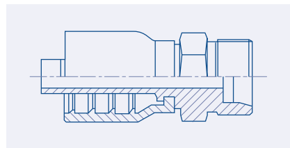
Heavy 24° Metric Male - DHM
