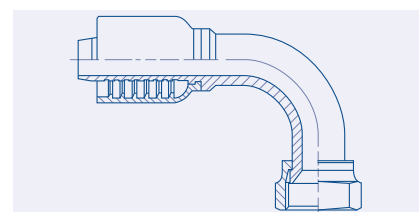
Female JIS 30° Swivel 90° Elbow - FX-KOMA90
