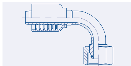
Heavy 24° Metric 90° Elbow Female - DHF90
