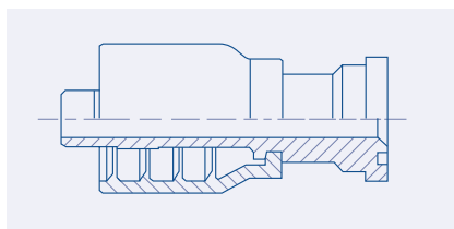
Straight SAE 6000 PSI Code 62 Flange - PH
