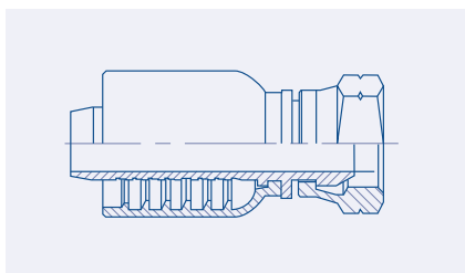
BSP 60° Swivel Female - BSPXF
