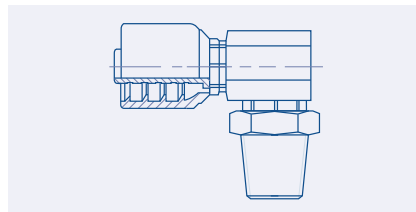
Male NPTF Swivel 90° Elbow - MPX90
