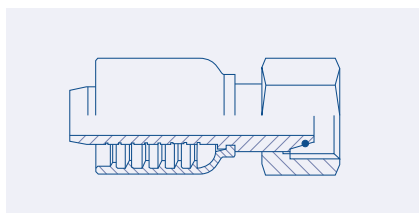
Light 24° Metric Female - DLF
