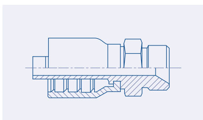
BSP 60° Male - BSPM
