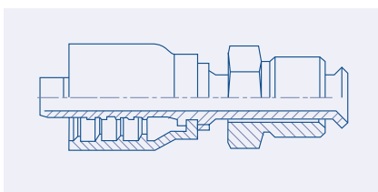
SAE Inverted 45° Flare Male - MSAE
