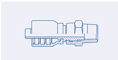
Male NPTF Swivel - MPX
