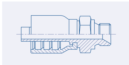
Light 24° Metric Male - DLM
