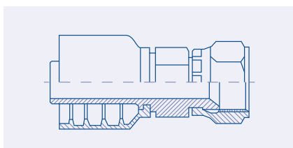
JIS 30° Female Swivel - FX-KOMA
