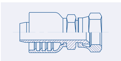
Female SAE 45° Swivel - FX
