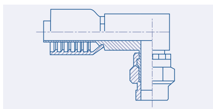
SAE 90° Elbow Swivel O-ring Boss Male - RAX90
