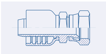
Female JIC 37° Swivel - FJ
