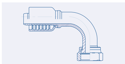
Female ORFS Swivel 90° Elbow - OFT90
