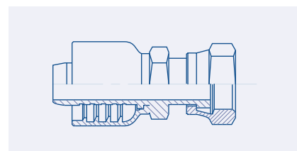
Female ORFS Swivel - OFT
