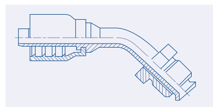
SAE Inverted 45° Flare 45° Elbow Male - MSAE 45
