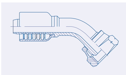
BSP 60° Swivel 45° Elbow Female - BSPXF45
